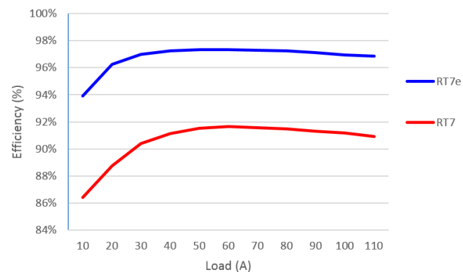
Efficiency at 380VAC/54VDC
